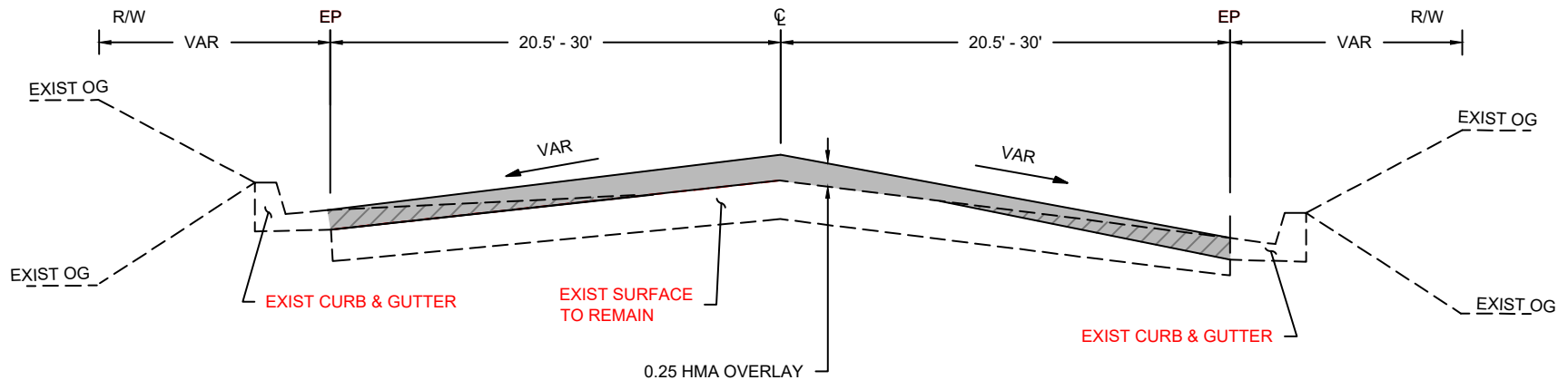
ASHLAN AVE - TYPICAL SECTION 0.04 MI W/O CLOVIS AVENUE TO 0.03 MI E/O SUNNYSIDE AVENUE
