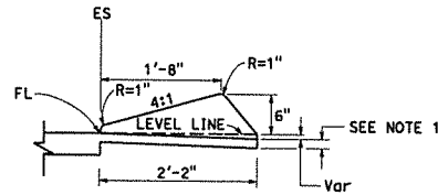
TYPE D DIKES
