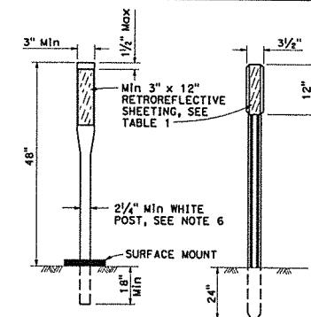
CLASS 1 FLEXIBLE POST DELINEATORS
