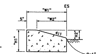
TYPE D CURBS See Table A
