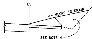
CASE C-2 Cut Slope
