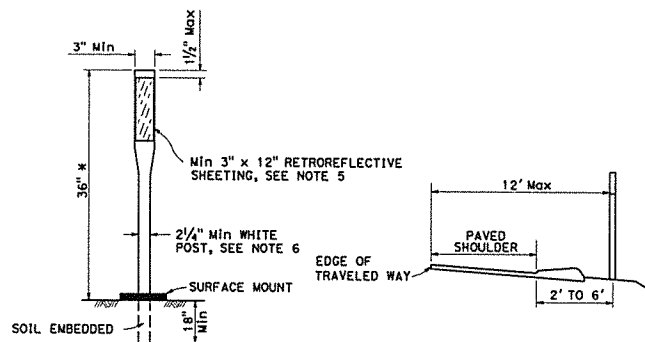
* 36" Min where speeds are 40 miles/h or less. CHANNELIZERS
