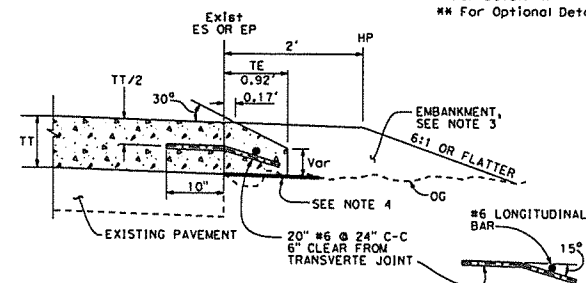
OPTIONAL DETAIL "A" For concrete overlay See Note 5
