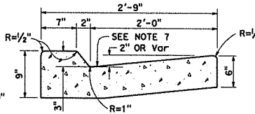
TYPE B4 CURBS
