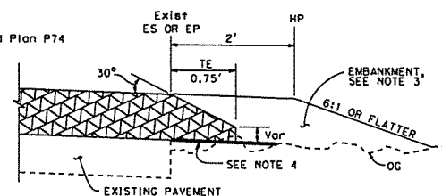
DETAIL "A" For HMA overlay thickness more than 0.43' or concrete overlay
