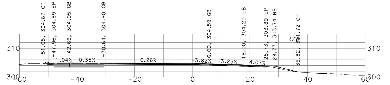
"GSB_R1_CL1" 76+00
