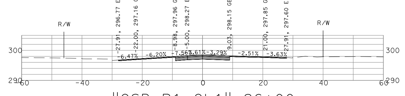
"GSB_R1_CL1" 26+00
