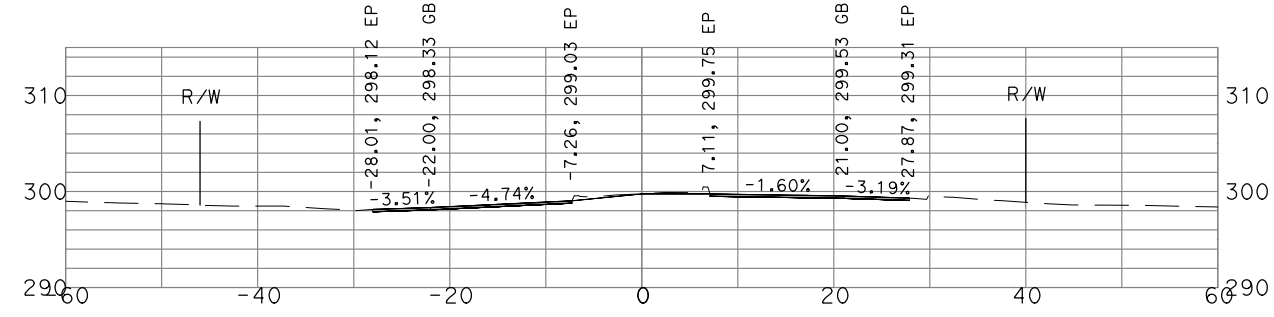
"GSB_R1_CL1" 37+00
