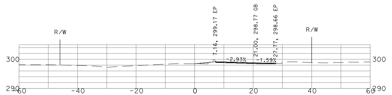
"GSB_R1_CL1" 33+00
