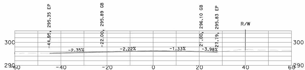
"GSB_R1_CL1" 13+50
