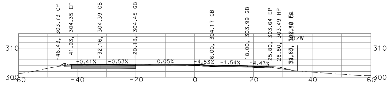
"GSB_R1_CL1" 74+50
