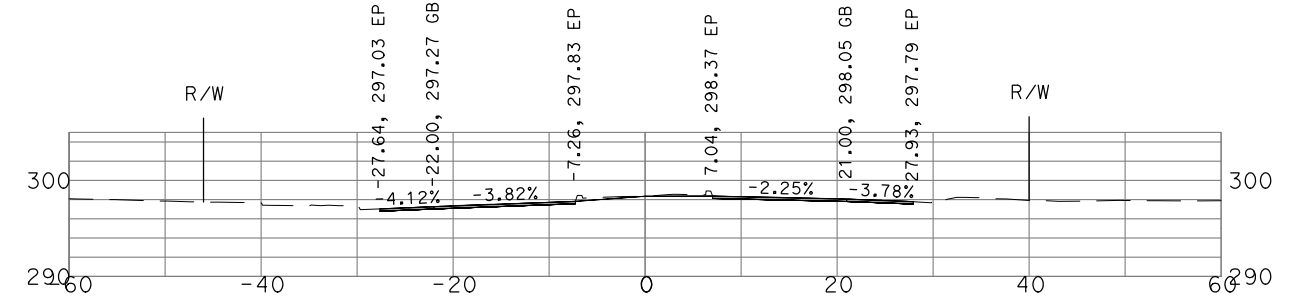
"GSB_R1_CL1" 27+50
