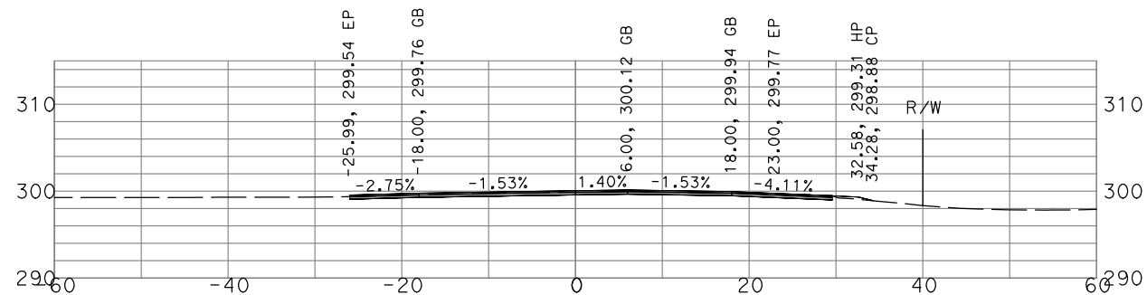
"GSB_R1_CL1" 53+00
