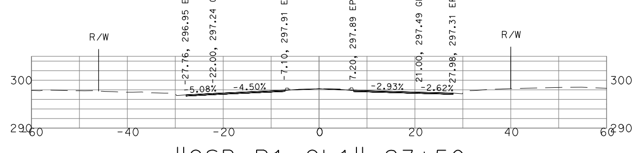
"GSB_R1_CL1" 23+50
