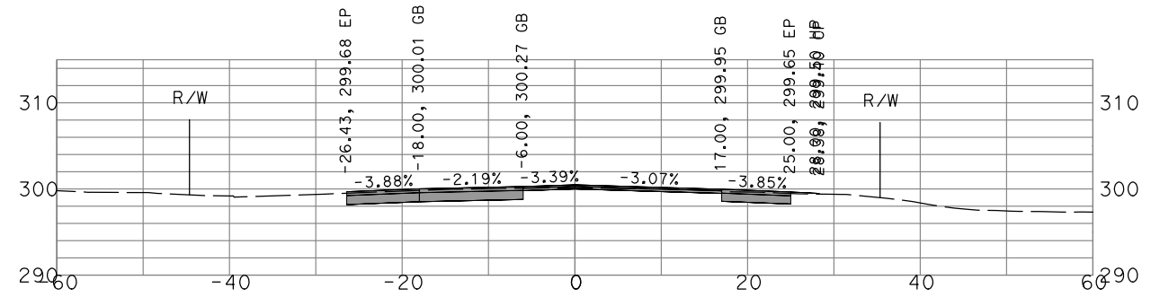
"GSB_R1_CL1" 60+50
