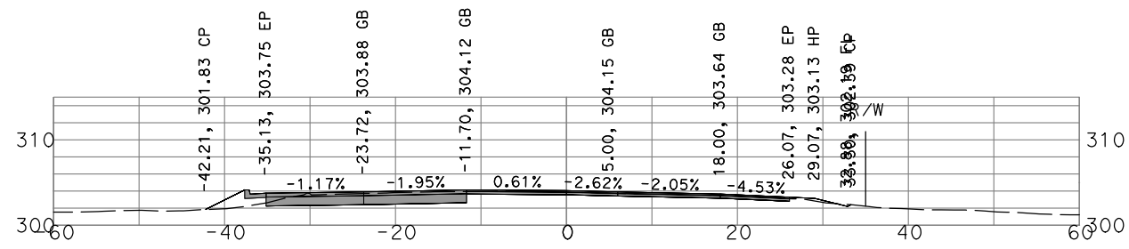
"GSB_R1_CL1" 73+00
