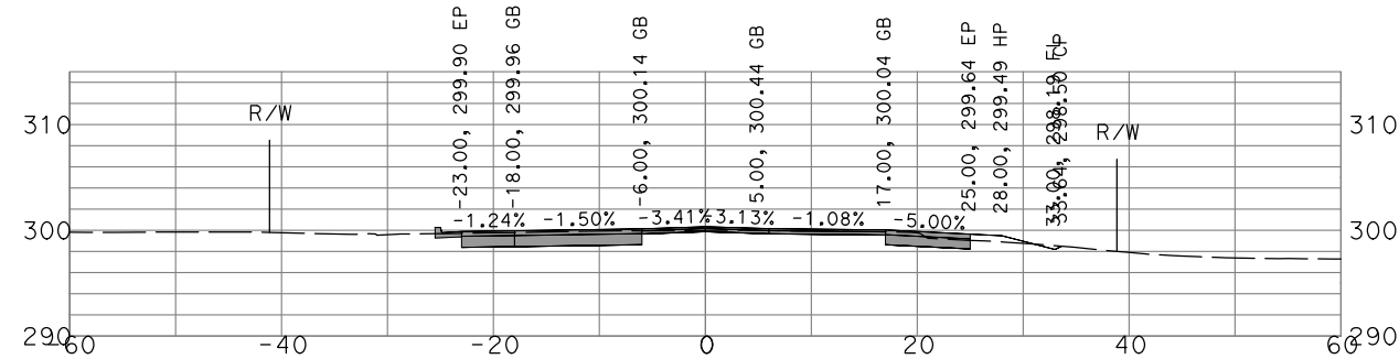
"GSB_R1_CL1" 55+50
