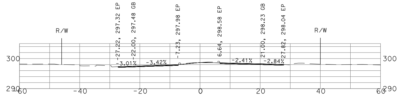
"GSB_R1_CL1" 28+50
