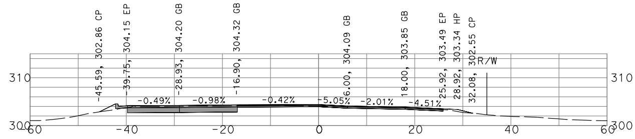
"GSB_R1_CL1" 74+00
