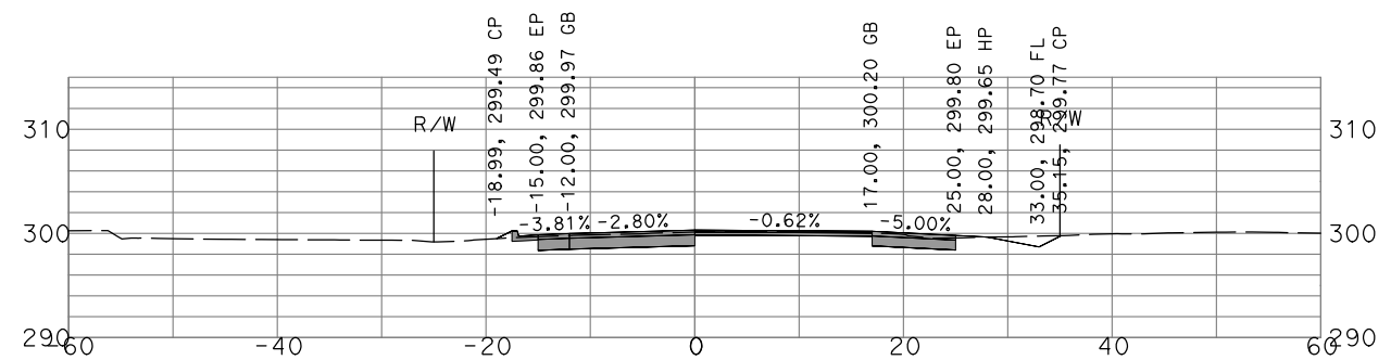
"GSB_R1_CL1" 67+00
