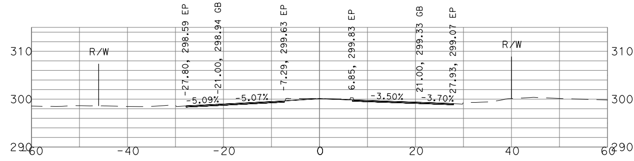
"GSB_R1_CL1" 46+50
