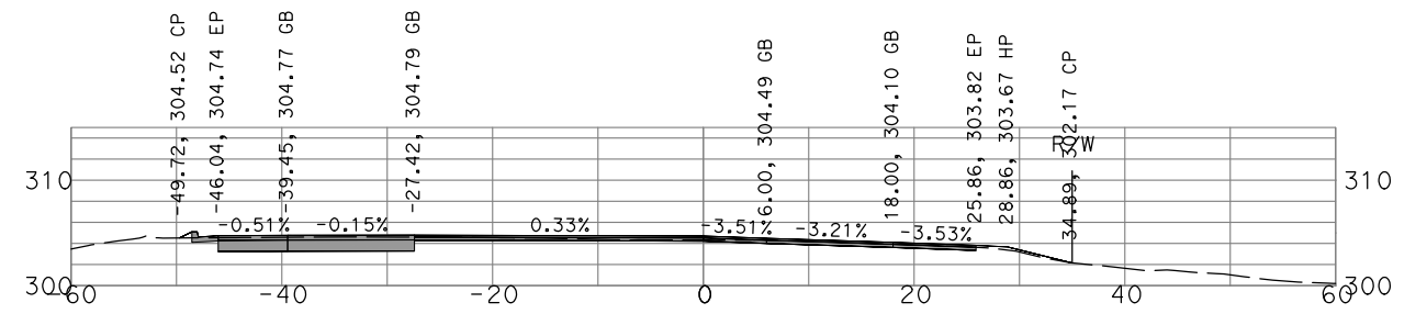
"GSB_R1_CL1" 75+50
