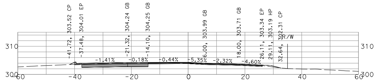
"GSB_R1_CL1" 73+50
