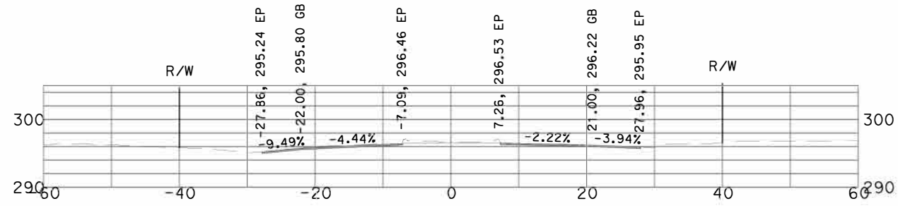
"GSB_R1_CL1" 14+50
