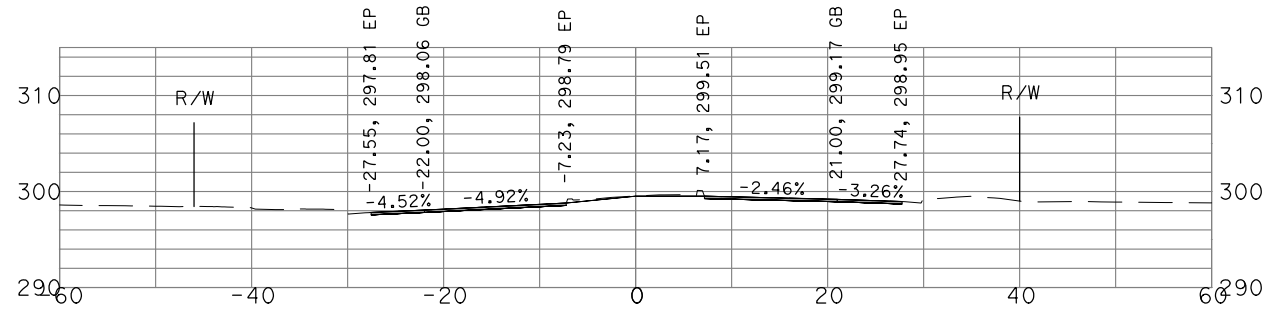
"GSB_R1_CL1" 35+00
