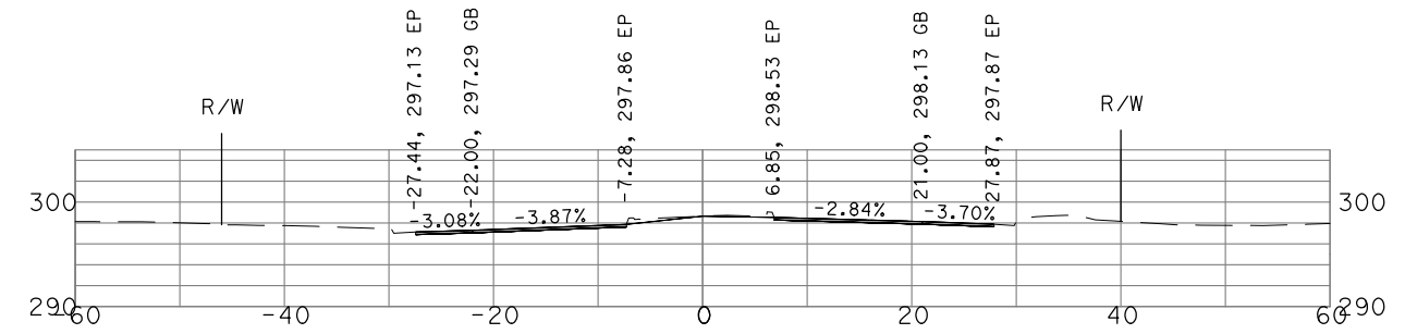
"GSB_R1_CL1" 28+00
