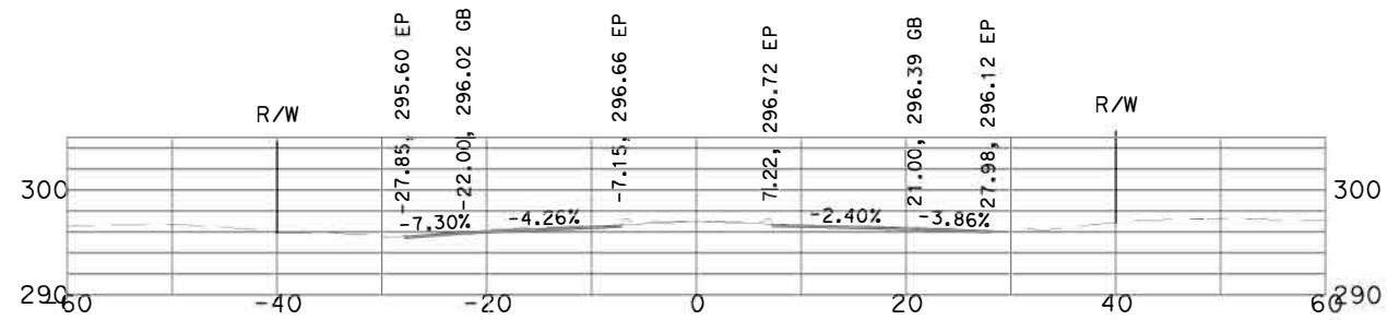
"GSB_R1_CL1" 15+50
