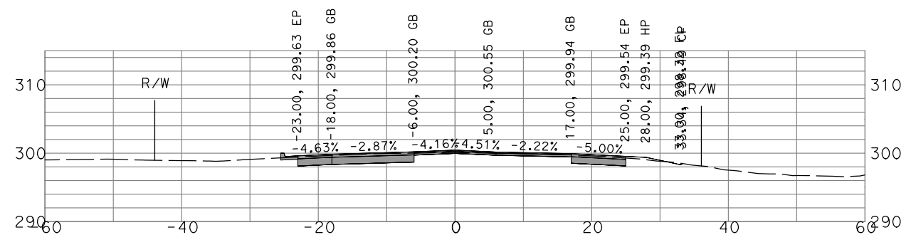
"GSB_R1_CL1" 59+50
