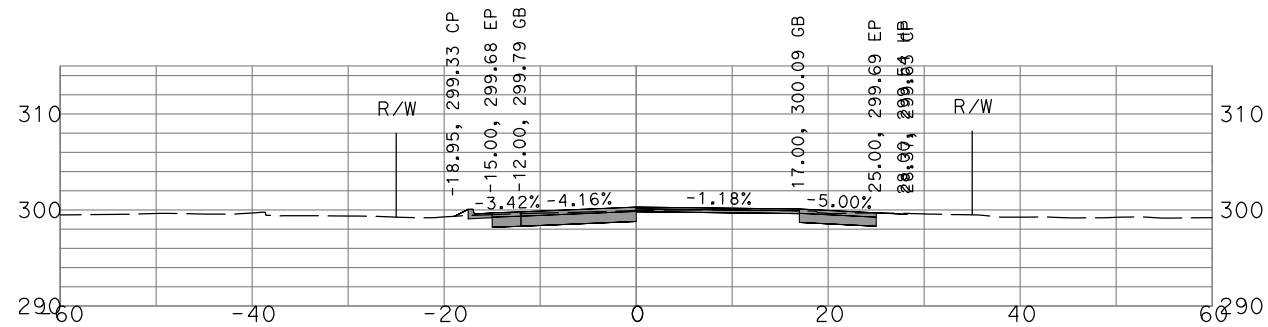
"GSB_R1_CL1" 66+00
