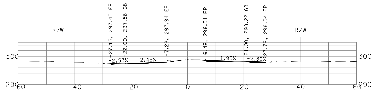
"GSB_R1_CL1" 29+00
