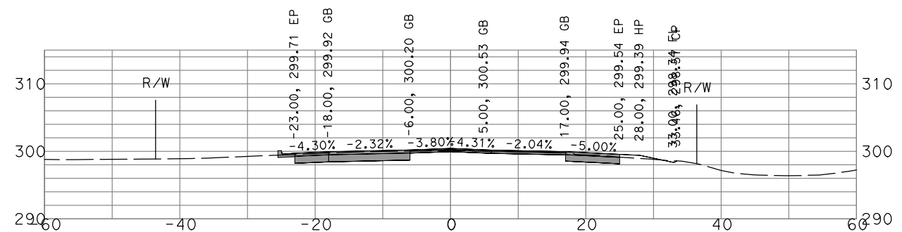
"GSB_R1_CL1" 59+00
