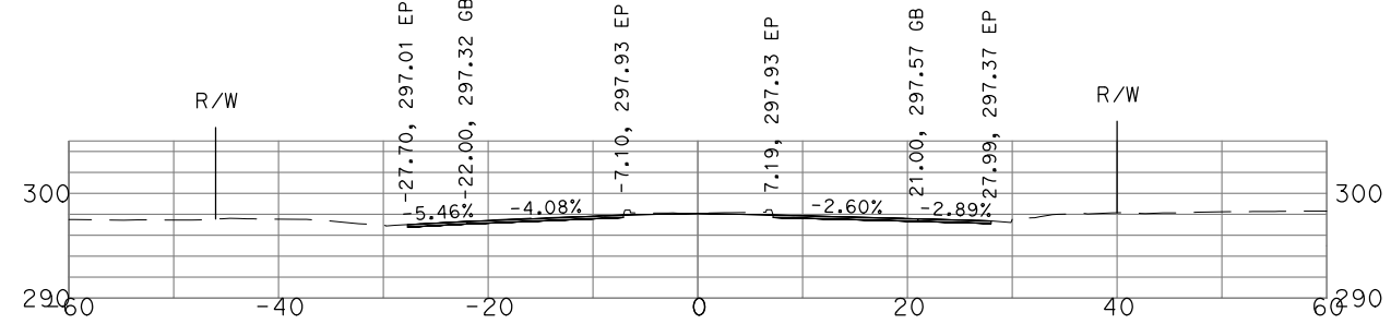
"GSB_R1_CL1" 24+00
