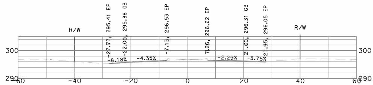
"GSB_R1_CL1" 15+00
