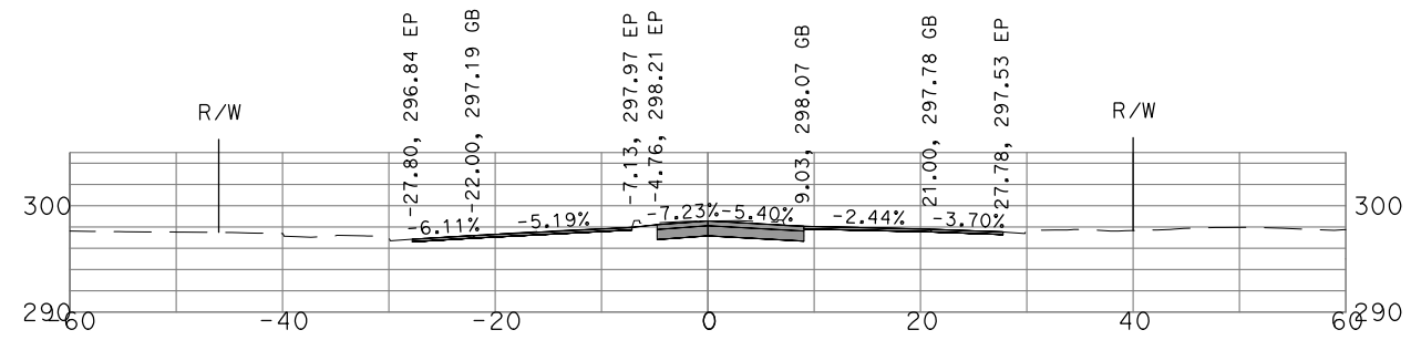
"GSB_R1_CL1" 25+50
