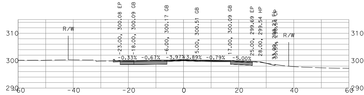
"GSB_R1_CL1" 56+50
