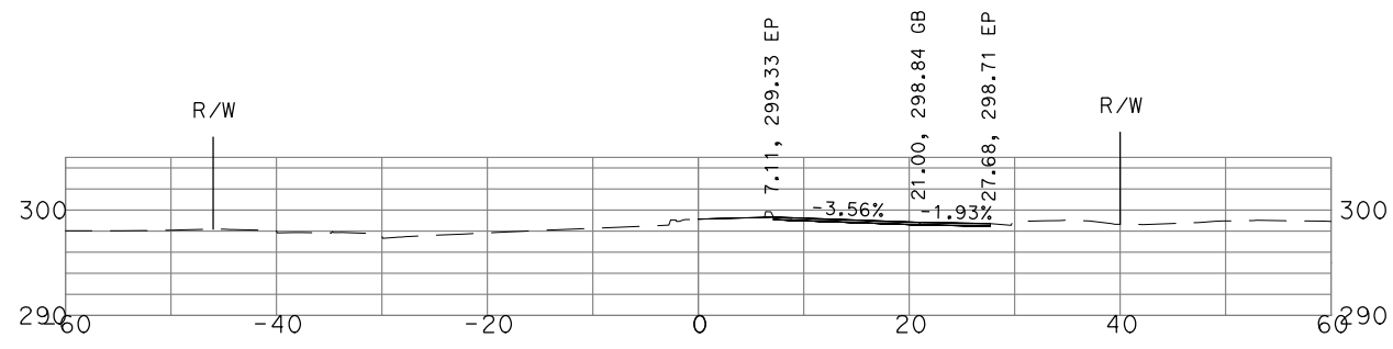
"GSB_R1_CL1" 33+50
