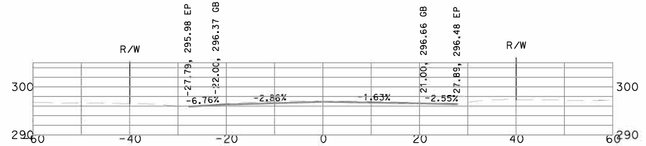
"GSB_R1_CL1" 17+50
