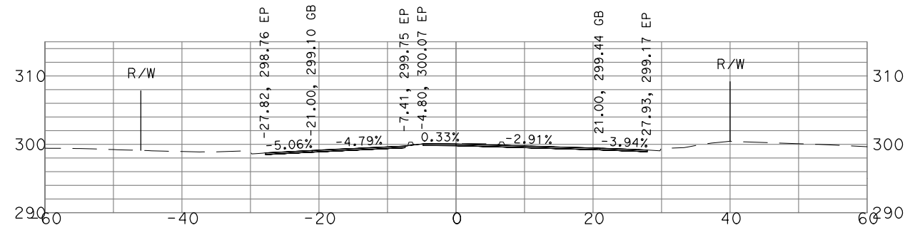
"GSB_R1_CL1" 45+50
