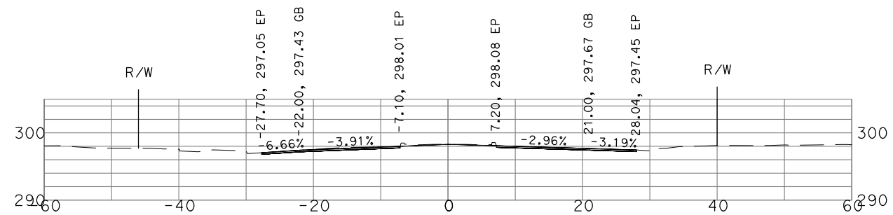
"GSB_R1_CL1" 24+50
