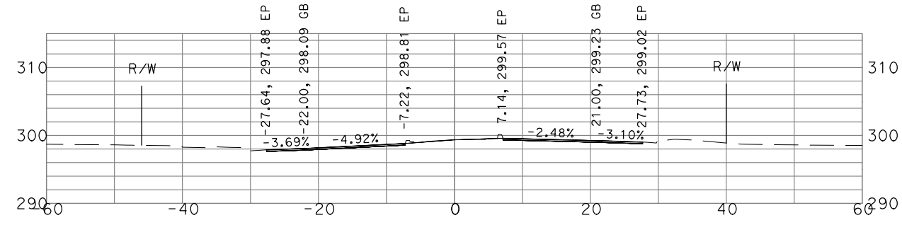
"GSB_R1_CL1" 35+50
