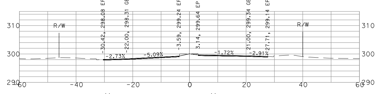
"GSB_R1_CL1" 36+00
