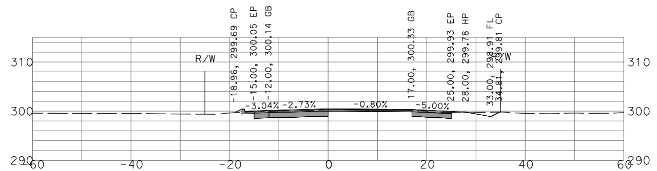
"GSB_R1_CL1" 67+50
