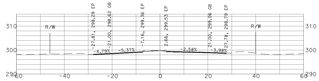
"GSB_R1_CL1" 49+00
