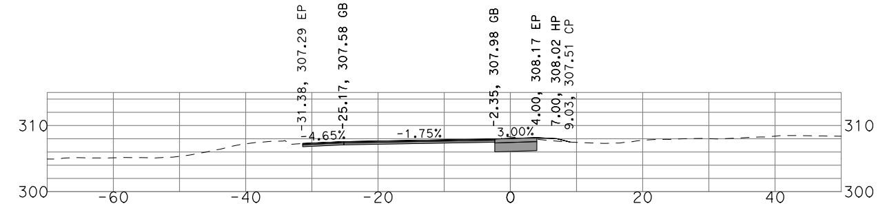
"GSB_R3_SB4" 525+50
