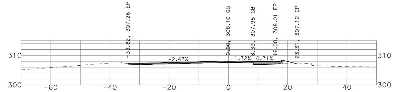
"GSB_R3_SB4" 472+00
