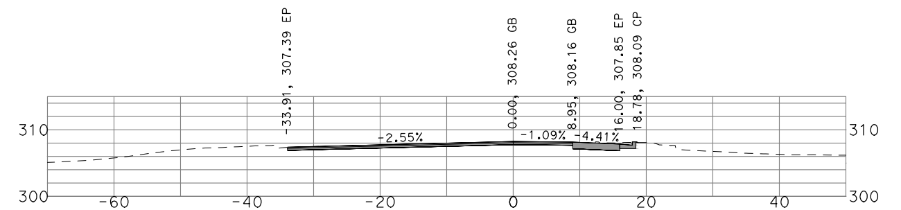
"GSB_R3_SB4" 471+50
