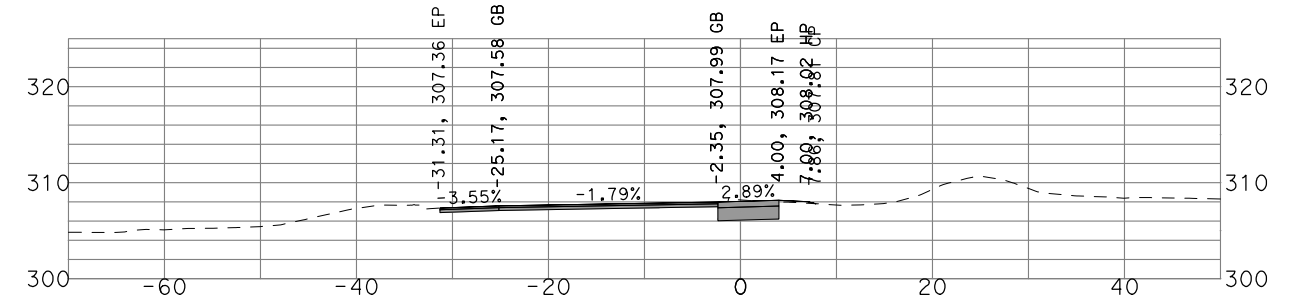
"GSB_R3_SB4" 526+00
