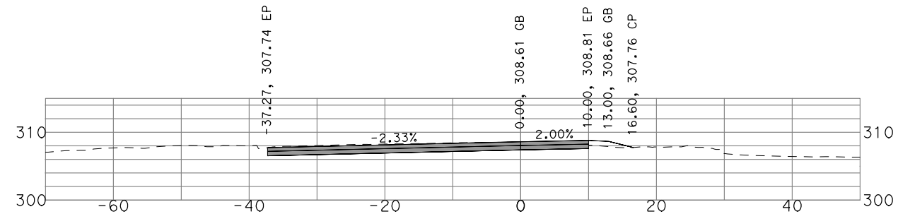
"GSB_R3_SB4" 470+00
