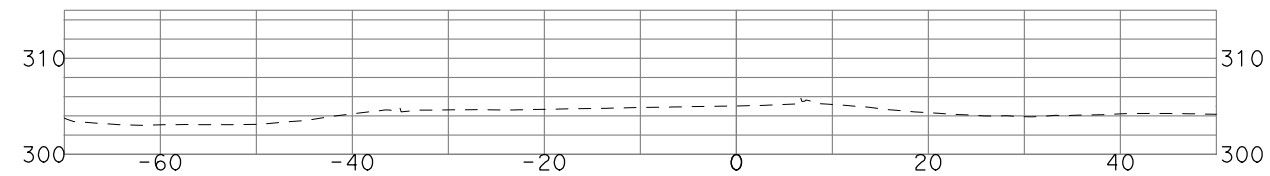
"GSB_R3_SB4" 482+00
