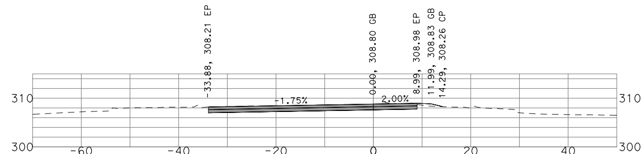
"GSB_R3_SB4" 469+50
