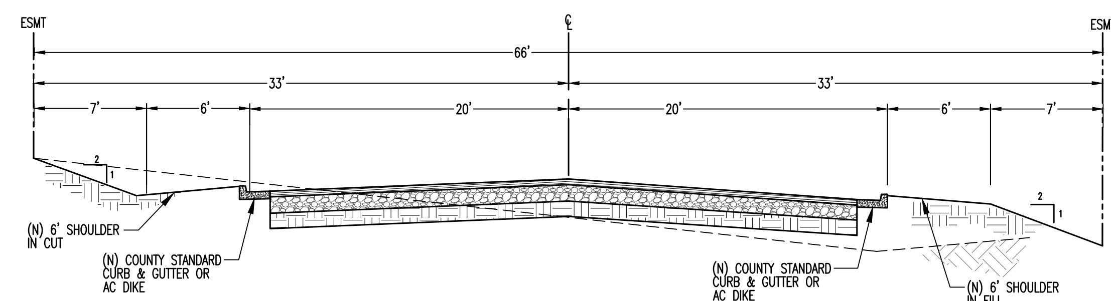
SECTION B - WILLOW AVE. ENTRY DRIVE SCALE: NTS
