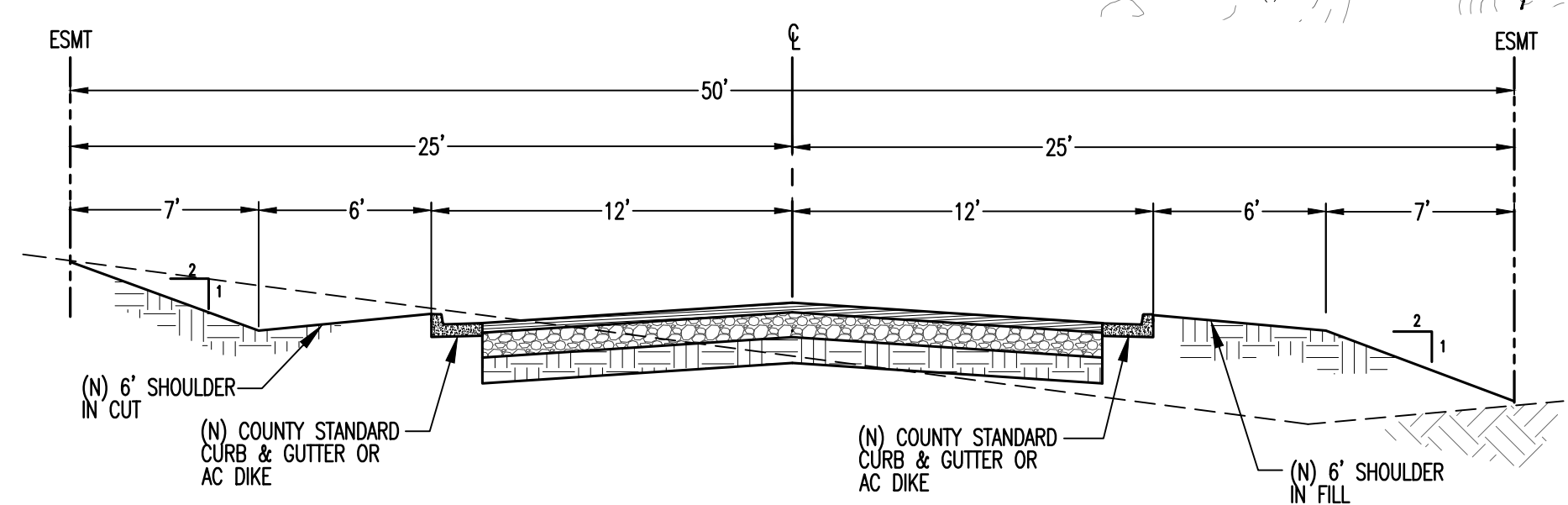
SECTION A - TYPICAL PUBLIC ACCESS SCALE: NTS
